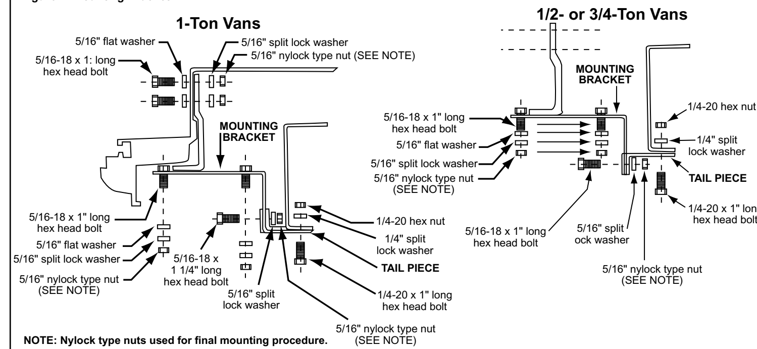
Figure 2: Mounting Bracket
